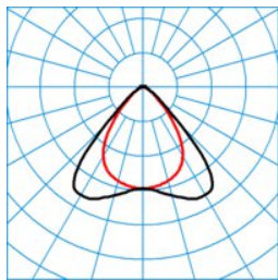
ELINE PW2255-120 ML 830 L225 2 50
