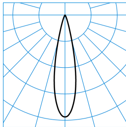
7651 Lentyp L-SP 40-EW M48 ETBLE 05 (150) TX782452
