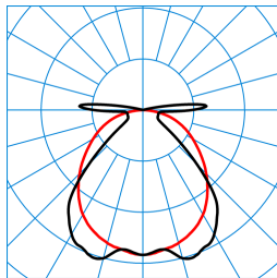
AragF 15 PW 64-840 ETDD +HFSB LV PC TX782238
