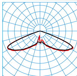
Publisca P1W-RB6L-LRA/2600-740 3G1S TX053548
