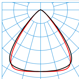
SFLOW C3-L LW19 40-830 ETBLE +CAS-S 01 TX562335
