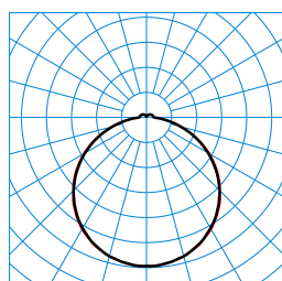
Olisq Act QWD3 DW 45 ETDD8 IP54 + Olisq QWD3 ZDR 1/2 01 (ACTDWW) TX461655
