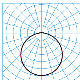
Olisq Act QWD3 DW 45 ETDD8 IP54 + Olisq QWD3 ZDR 1/2 03 (ACTDWW) TX461162
