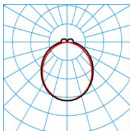
ELINE DSL50-130 ML 865 L225 2 50
