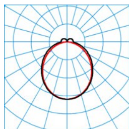
ELINE DSL50-130 ML 865 L225 0 50
