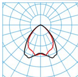
ELINE HE LW60 827 L150 2 20
