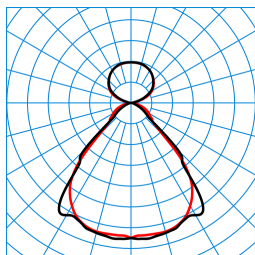
SFlow-Act H3-L MRW LED6400 ETDD8 LLWS 01 (ActDSU) TX299675
