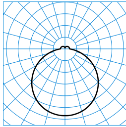
Olisq Act RWD2 DW 20 ETBLE +CAS-S IP54 (ACTDSU) TX565667
