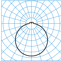
Olisq Act RWD2 DW 20 ETBLE +CAS-S IP54 (ACTDCW) TX565666
