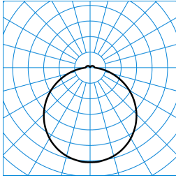
Olisq Act RWD2 DW 20 ETBLE +CAS-S IP54 + Olisq RWD2 ZDR 1/2 05 (ACTDWW) TX565689
