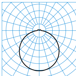
Olisq Act RWD2 DW 20 ETBLE +CAS-S IP54 + Olisq RWD2 ZDR 1/2 03 (ACTDWW) TX565686
