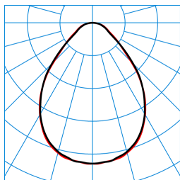
ArimoFit G2 Act D PW19 42-8 ETBLE +CAS (ACTDSU) TX559862
