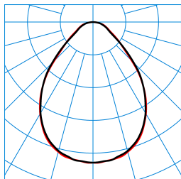
ArimoFit G2 Act D PW19 42-8 ETBLE +CAS (ACTDCW) TX559808
