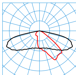
LIQ 50N-AB2L-LR/1650-727 2G1 ET (CLO initial value) TX776388
