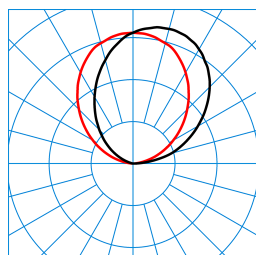
Sanesca W4-L20/R LED5300-830 ET 03 (night light) TX772948
