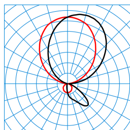
Sanesca W4-L20/R LED5300-830 ET 03 (B) TX772945
