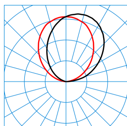
Sanesca W4-L20/R LED5300-830 ET 03 (room light) TX772954
