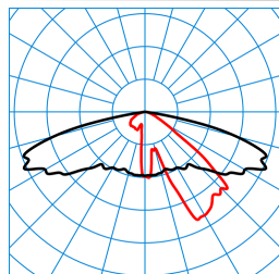
Publisca P1W-AB2L-LRA/1200-740 2G1S TX053492
