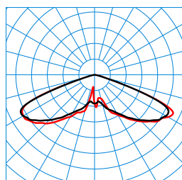
Publisca P1-RB6L/2000-730 3G1S ETDD (CLO end value) TX301707
