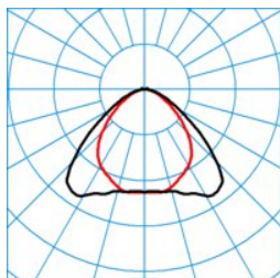
ELINE HE LVW60-160 ML 840 L225 4 20 ■ C0 - C180
