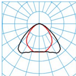
ELINE HE LVW60-160 ML 840 L225 2 20 ■ C0 - C180
