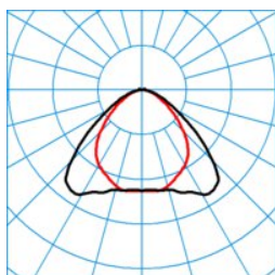
ELINE HE LVW60-160 ML 840 L225 0 20 ■ C0 - C180
