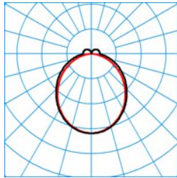
ELINE DSL50-130 ML 830 L225 2 20
