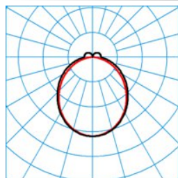
ELINE DSL50-130 ML 830 L225 0 20
