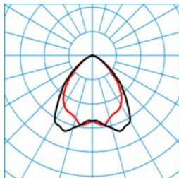
ELINE HE LW40-120 ML 840 L150 0 50 ■ C0 - C180
