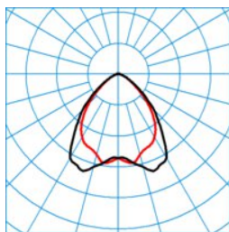
ELINE HE LW40-120 ML 840 L150 2 50 ■ C0 - C180
