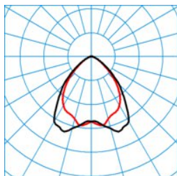
ELINE HE LW40-120 ML 840 L150 4 50 ■ C0 - C180
