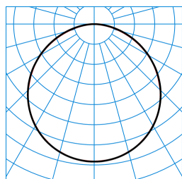
Siella G8 M84 DW 28-40/3ML-8MC ET (stage 4) TX562653
