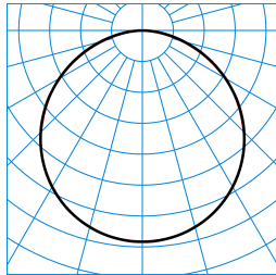
Siella G8 M84 DW 28-40/3ML-8MC ET (stage 6) TX562647
