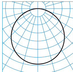
Siella G8 M84 DW 28-40/3ML-8MC ET (stage 1) TX562677
