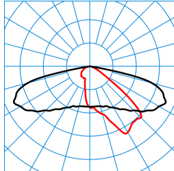
LIQ 50N-AB2L-LR-SLR2/4200-727 4G1 ET (CLO end value) TX777106
