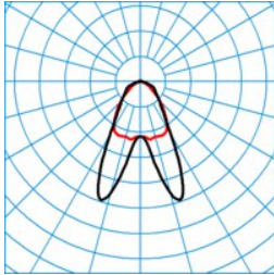
ELINE HE LDAN40-120 ML 840 L150 2 50 ■ C0 - C180
