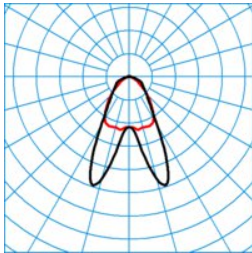
ELINE HE LDAN40-120 ML 840 L150 4 50 ■ C0 - C180
