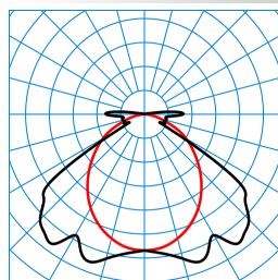
Nextrema G3 B 60-840 ETDD +HFSB LV TWP TX768230
