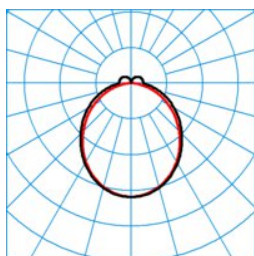
ELINE HE DSL35-110 ML 840 L150 0 50
