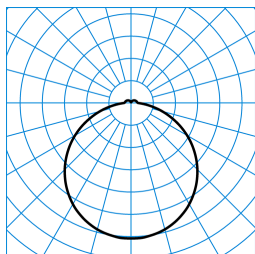
Olisq RWD2 DW 20-830 ETBLE +CAS IP54 + Olisq RWD2 ZDR 1/2 03 TX565844
