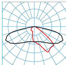
LIQ 50N-AB2L-LR/4200-730 4G1 ET (CLO end value) TX777862
