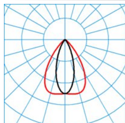
ELINE HE LVN40-120 ML 830 L150 0 20 ■ C0 - C180
