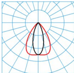
ELINE HE LVN40-120 ML 830 L150 4 20 ■ C0 - C180
