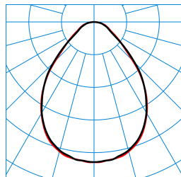
ArimoFit M48 PW19 53-840 ET + ArimoFit Sky M48-TS ZER TX426324
