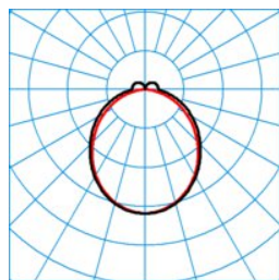
ELINE DSL50-130 ML 830 L225 2 50
