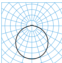
Olisq Act RWD2 DW 40 ETDD8 IP54 PC + Olisq RWD2 ZDR 1/2 03 (ActDWW) TX427717
