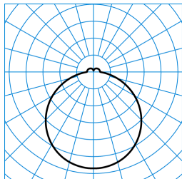
Olisq Act RWD2 DW 40 ETDD8 IP54 PC (ActDWW) TX376108
