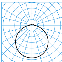
Olisq Act RWD2 DW 40 ETDD8 IP54 PC (ActDSU) TX375947
