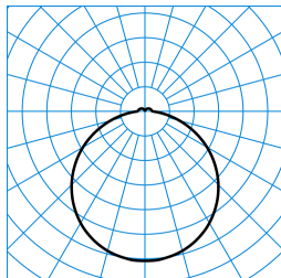
Olisq Act RWD2 DW 40 ETDD8 IP54 PC + Olisq RWD2 ZDR 1/2 05 (ActDWW) TX428621
