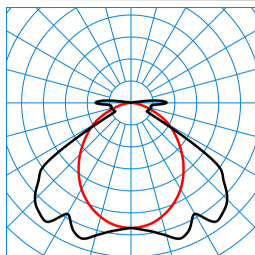
Nextrema G3 HE B 40-840 ETDD TWP PC TX768273
