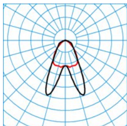
ELINE HE LDAN60-160 ML 830 L225 4 20 ■ C0 - C180
