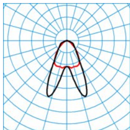
ELINE HE LDAN60-160 ML 830 L225 2 20 ■ C0 - C180
