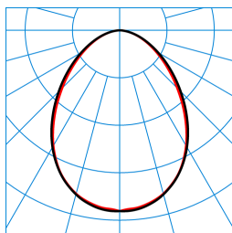
SFlow C1-L MRWD LED3200-830 ETDD 01 TX721353
