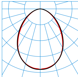
SFlow C1-L MRWD LED3200-830 ETDD 01 TX771460
