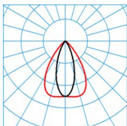
ELINE HE LVN60-160 ML 830 L225 0 50 ■ C0 - C180
