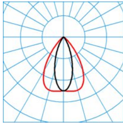
ELINE HE LVN60-160 ML 830 L225 2 50 ■ C0 - C180
