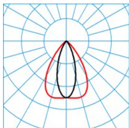
ELINE HE LVN60-160 ML 830 L225 4 50 ■ C0 - C180
