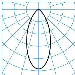
Skeo Q-D2 GS RB12R/2500-830 ETDD TX773677
