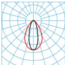
ELINE PN35-110 ML 840 L150 4 50
