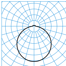
Olisq Act RWD4 DW 40 ETBLE +CAS-S IP54 (ACTDSU) TX565526
