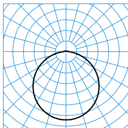
Olisq Act RWD4 DW 40 ETBLE +CAS-S IP54 + Olisq RWD4 C 01 (ACTDWW) TX565529
