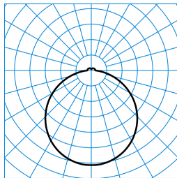
Olisq Act RWD4 DW 40 ETBLE +CAS-S IP54 (ACTDWW) TX565527
