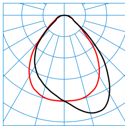
ArimoFit G2 Act M59 P-WW 53-8 ETDD8 (ActDCW) TX376493
