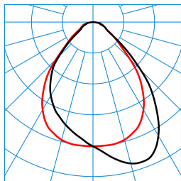
ArimoFit G2 Act M59 P-WW 53-8 ETDD8 (ActDWW) TX376408
