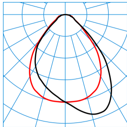
ArimoFit G2 Act M59 P-WW 53-8 ETDD8 (ActDSU) TX376409
