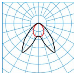
ELINE LDAW40-110 ML 830 L150 4 50
