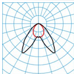
ELINE LDAW40-110 ML 830 L150 0 50
