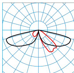
CS 19 100-AB2L/4600-740 4G1S ETDD (CLO initial value) TX300025
