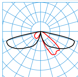
CS 19 100-AB2L/4600-740 4G1S ETDD (CLO end value) TX300024
