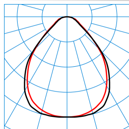
ArimoFit Act M48 PW19 53-8 (ActDWW) TX149843
