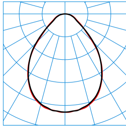
ArimoFit Act M48 PW19 53-8 ETDD8 + ArimoFit Sky M48-TS ZER (ActDCW) TX426308
