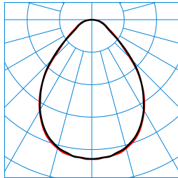
ArimoFit Act M48 PW19 53-8 ETDD8 + ArimoFit Sky M48-TS ZER (ActDSU) TX426309
