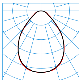
ArimoFit Act M48 PW19 53-8 ETDD8 + ArimoFit Sky M48-TS ZER (ActDWW) TX426310
