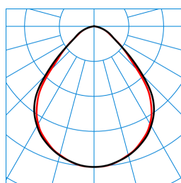
Opendo D2-L PW19 20-47/5/ML-830 ET 03 (3300lm) TX376586
