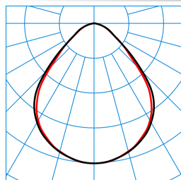
Opendo D2-L PW19 20-47/5/ML-830 ET 03 (1900lm) TX376583
