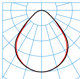
Opendo D2-L PW19 20-47/5/ML-830 ET 03 (2400lm) TX376581
