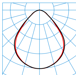
Opendo D2-L PW19 20-47/5/ML-830 ET 03 (2900lm) TX376580
