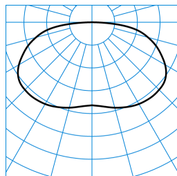
PolaronIQ WD1-2D LED3000-830 + WD2 C1 TX773772
