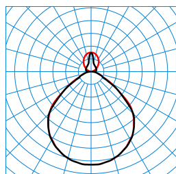
Luceos D/H1-L CDP 4000-830 01 (Ceiling D1 ZD/01) TX194590
