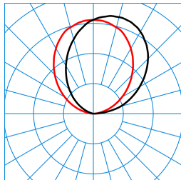
Sanesca W3-S1/R LED5000-830 03 (night light) TX055778
