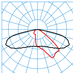
LIQ 50N-AB2L-LRA/4200-740 6G1 ETDD (CLO end value) TX779073
