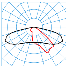
LIQ 50N-AB2L-LRA/4200-740 6G1 ETDD (CLO initial value) TX779079
