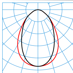
ArimoFit G2 M57 DW19 IP 42-840 ET TX376476
