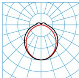
ELINE DL50-130 ML 840 L225 4 50
