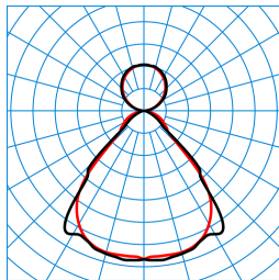
SFlow H2-L MRW LED6400-830 ET 01 TX770245
