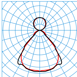
SFlow H2-L MRW LED6400-830 ET 01 TX721257
