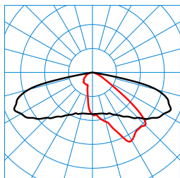
LIQ 50N-AB2L-LR/3200-722 4G1 ET (CLO initial value) TX777716
