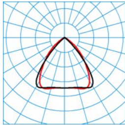
ELINE HE LN60-160 ML 830 L225 2 50
